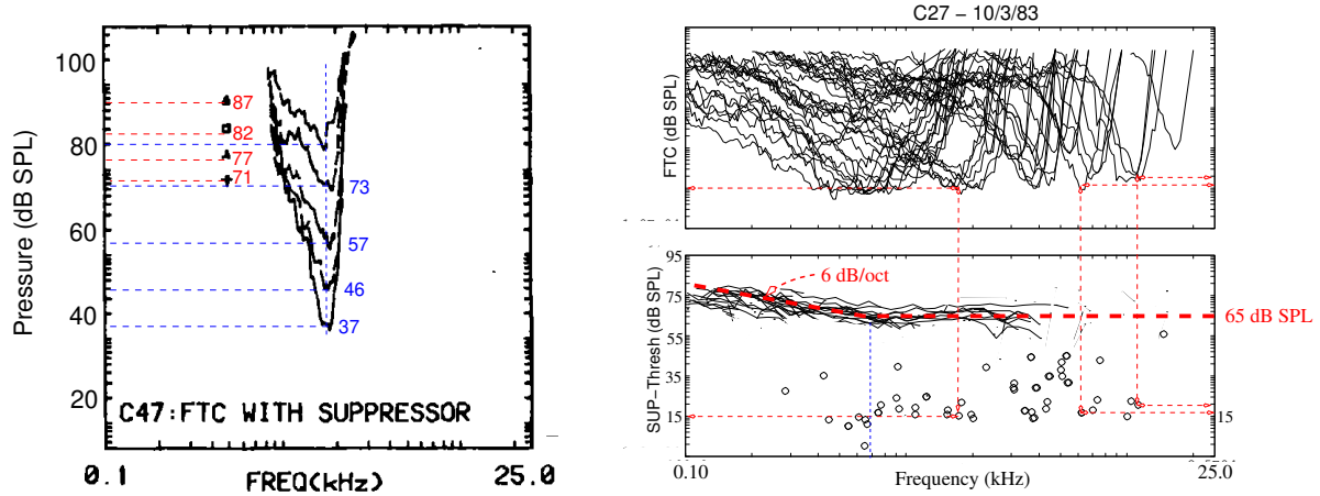
Figure 2: Data from FA-85 FaheyAllen85, animals #47 and #27. Compare this with Fig. 6 of Allen90b.
