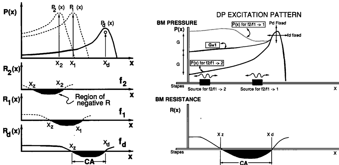
Figure 1: These cartoon figures from Allen92a(1992) describe the experimental protocol for measuring the cochlear amplifier gain on the basilar membrane. In the LEFT panel two tones at frequencies f_1 < f_2 excite the cochlear OHC cilia in the overlapping region X_1(f_1) > X_2(f_2) . In this way the experiment excites neurons tuned to f_d at X_d(f_d) from the small region between X_1 > X_2 . The experimental goal is to record the threshold neural response at X_d(f_1, f_2) .
